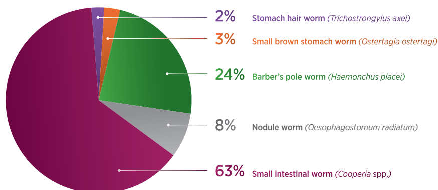
Proportion of species by worm egg counts found in cattle in South-West Qld, Alice Springs and Pilbara region of WA
